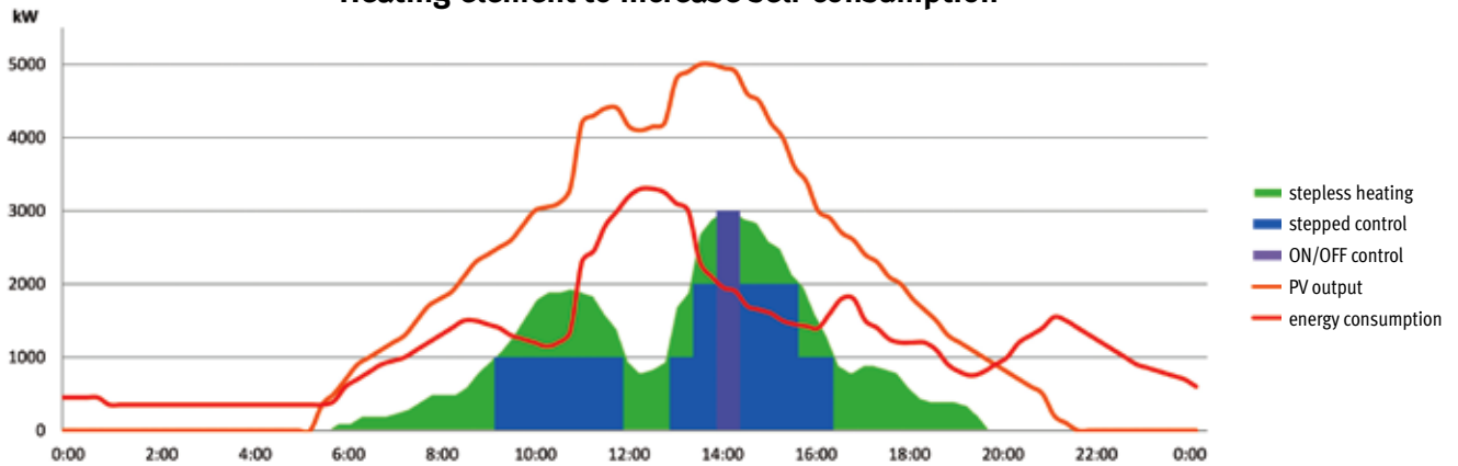
Fig. 1: A stepless heating element converts much more PV energy into heat than a 1- or 3-step one.
